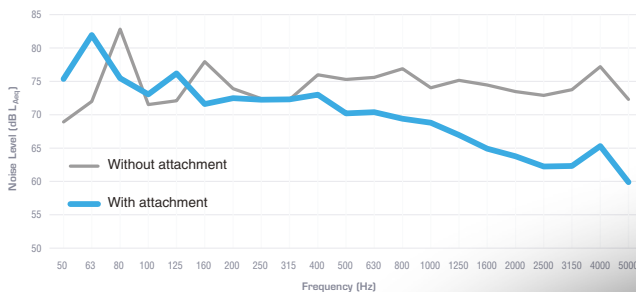
THIRD OCTAVE BAND SPECTRA FOR MEASUREMENTS
